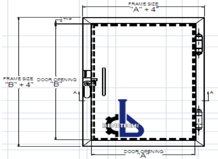
ELEVATION VIEW NOTE: DOOR IS PRIMERED AND PAINTED SAFETY YELLOW
