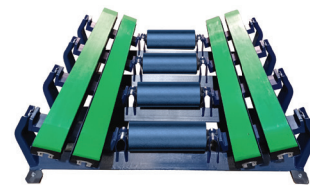
Support & Seal Bed
