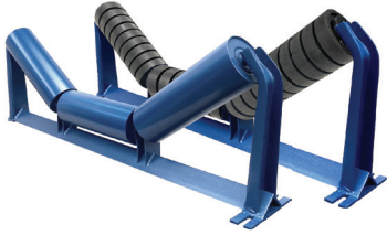
Steel & Impact Troughing Idlers
