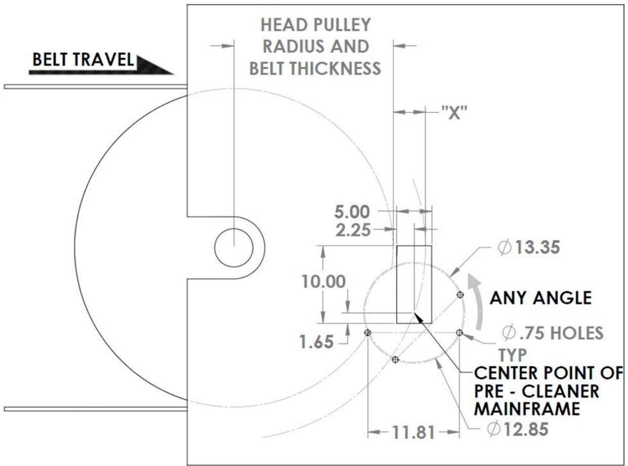
Figure 4: Hole Cutout Template
